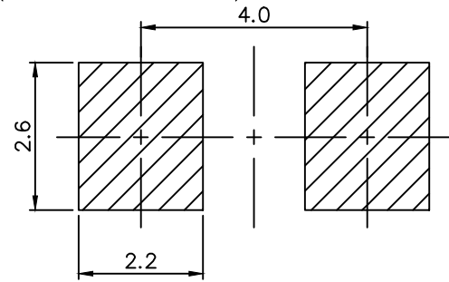
RECOMMENDE PCB LAYOUT
