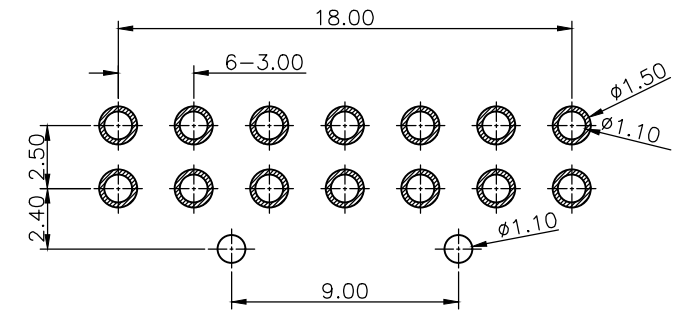
RECOMMEND PCB LAYOUT(TOP VIEW) Layout Tolerance: ± 0.05mm
