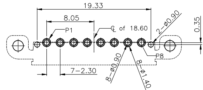
RECOMMEND PCB LAYOUT(TOP VIEW) Layout Tolerance: ± 0.05mm
