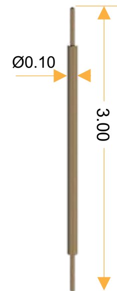
Pitch 0.20mm
