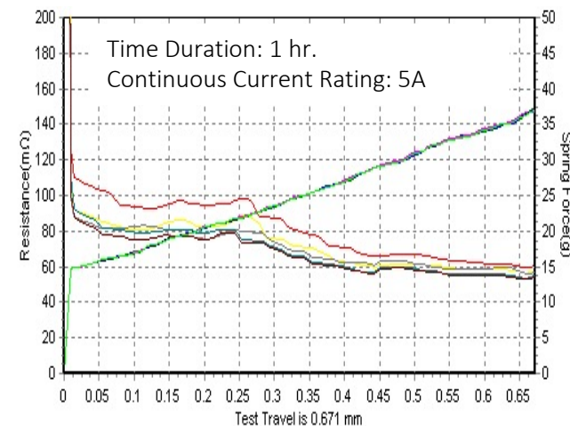
High Current Testing
